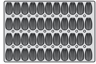
74102-07 MADELEINE 44 cav. 78 x 45 x 18 mm. / 3,07" x 1,77" x 0,71"
