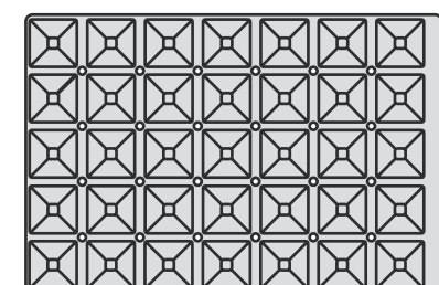
74102-01 PYRAMIDE 35 cav. 68 x 68 x 35 mm. / 2,68" x 2,68" x 1,38"
